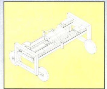
Parallel Vacuum Gripper for Large Box Handling.
