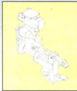
O.D. Gripper with Air Motor Power Rotate.
